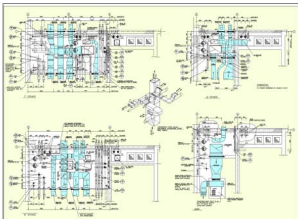
Shaft Duct and Piping Details and Isometrics
