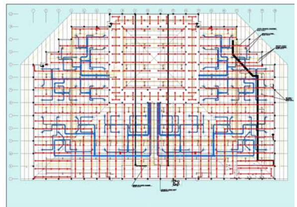
Composite HVAC, FP, Lighting and Systems Plan
