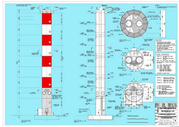
Kos Island Power Plant Stack
