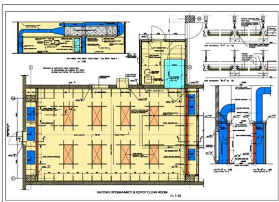
Missile Components Clean Room 10 000 Class
