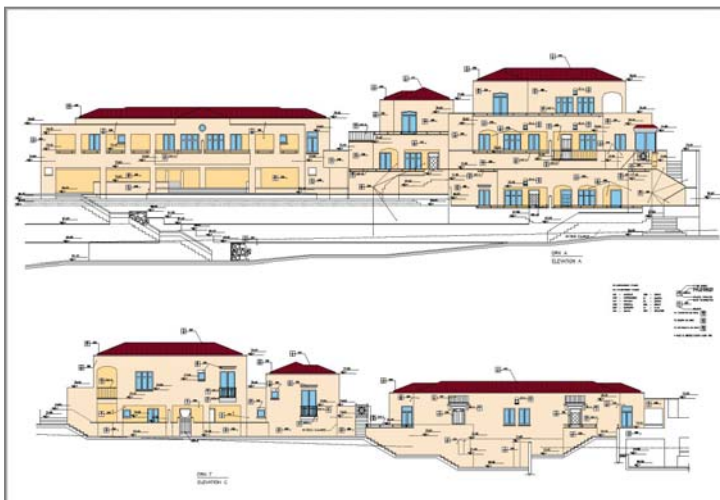
Reousa Maria Resort Housing Complex –Partial Elevation
