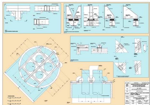
Paros Island Power Plant Stack
