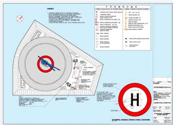
Headquarters Office Building- Roof Helipad
