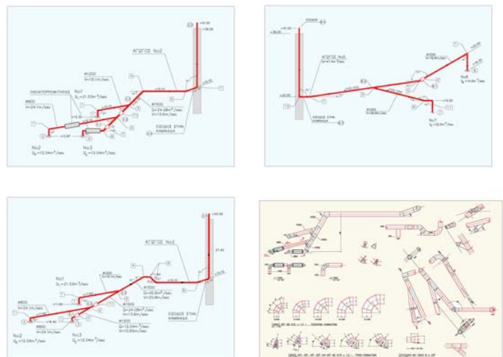
Paros Island Power Plant Exhaust Ducts Isometrics
