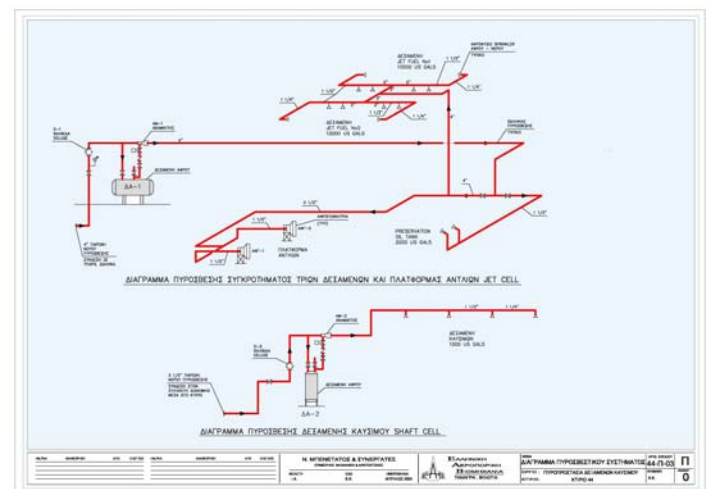
Jet Fuel Storage Tanks Fire Protection Piping Isometrics
