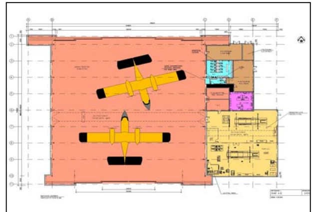
Aircraft Hangar – Floor Plan
