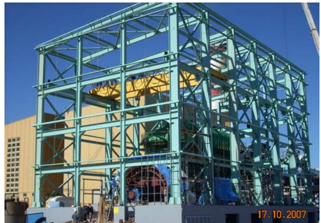
Chios Turbine House – Unit No. 3
